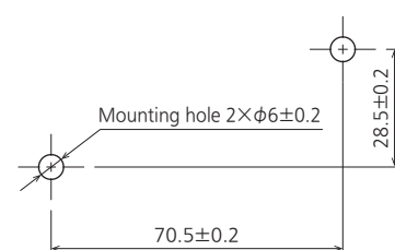
Mounting dimensions
